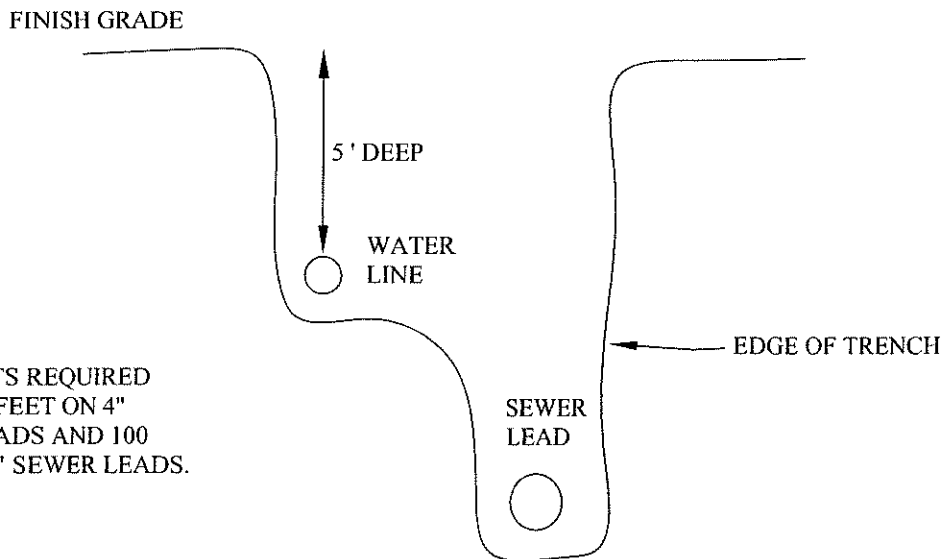
PROFILE VIEW
